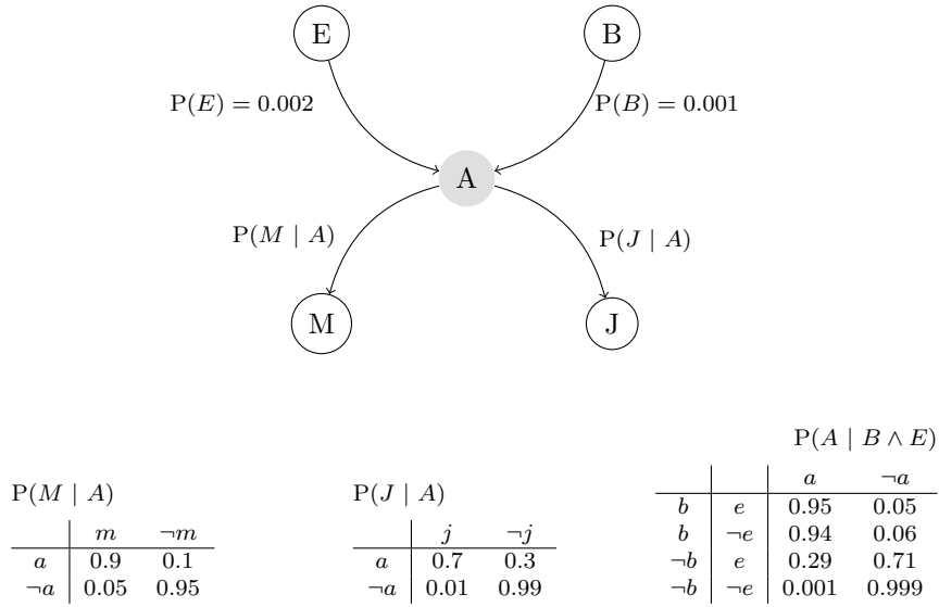
Figure 3: The Earthquake, Burglary, Alarm model
